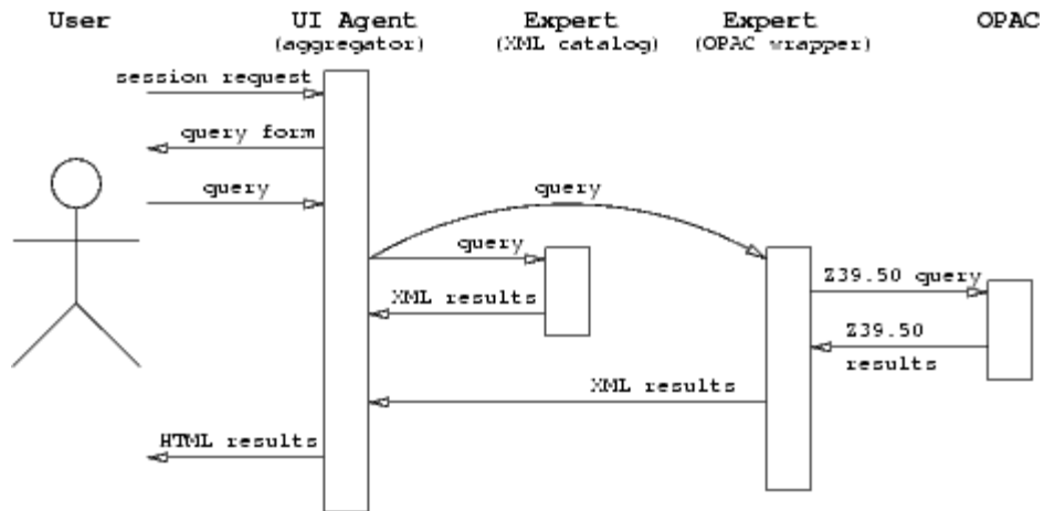
Fig. 2: Sequence Diagram
